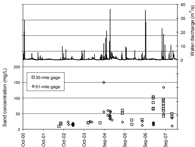
Figure 4. Paria River water discharge (top) and mainstem Colorado River sand concentrations for mainstem discharges in the 322 m 3 /s ±5% range (bottom) for October 2000–April 2008. Sand concentrations increased during temporary sand accumulation in Marble Canyon following Paria floods in fall 2004, winter 2005, and fall 2006 and subsequently decreased as the tributary sand was exported from Marble Canyon.
